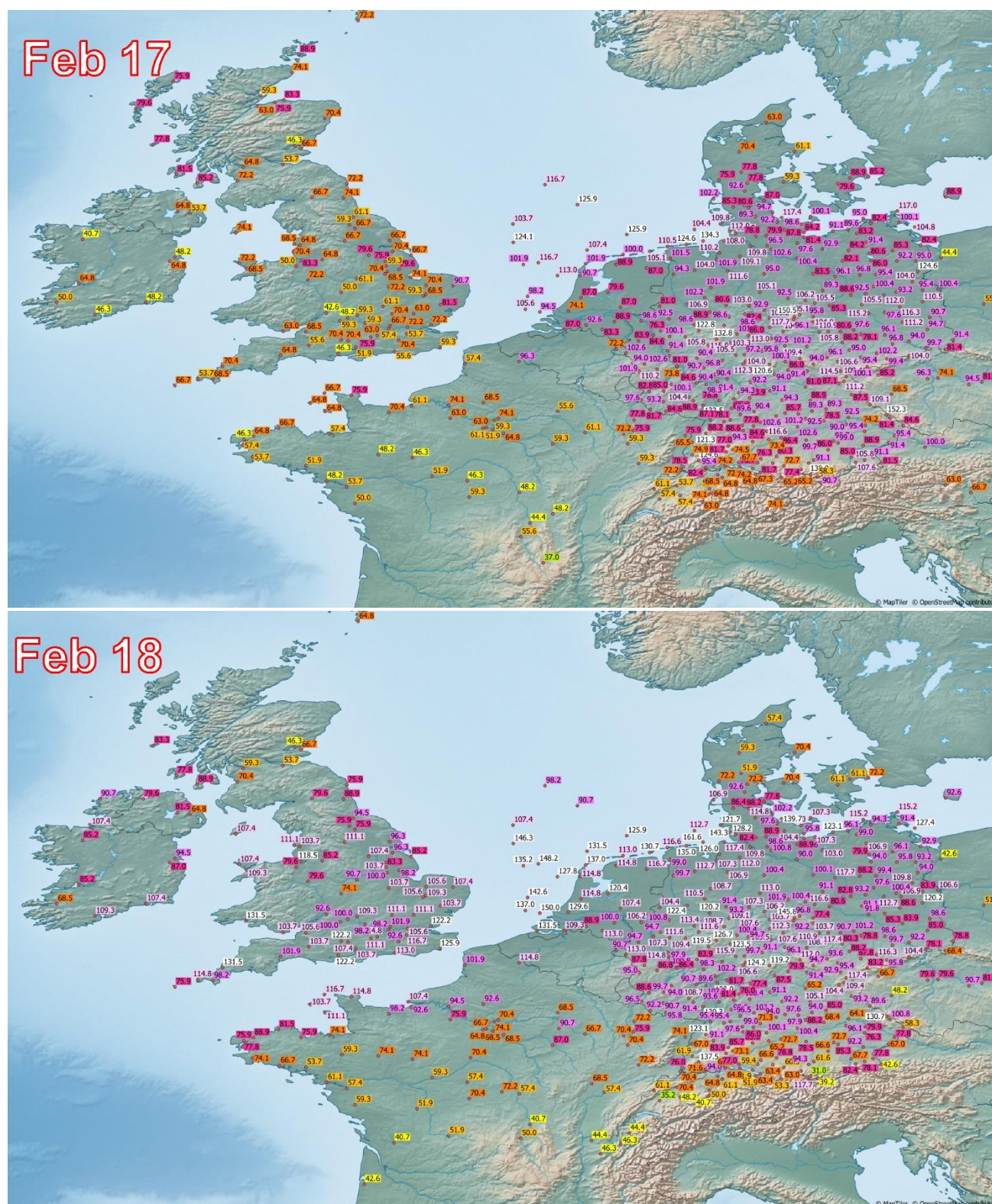
Figure 7b: Maximum wind gusts (German weather station network of DWD and METARS), Feb 17 2022 (top) and Feb 18 2022 (bottom). Data source: DWD and http://www.mesonet.agron.iastate.edu
