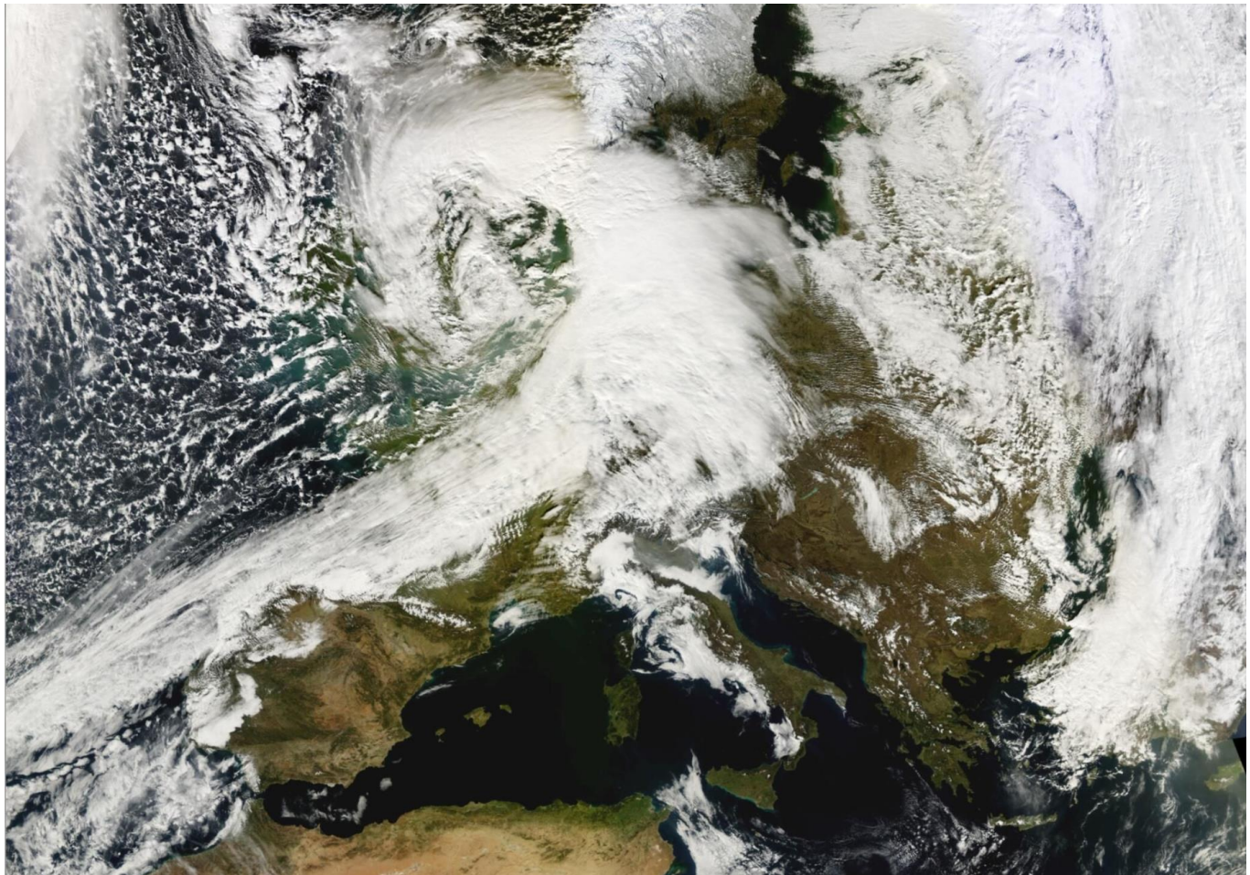
Figure 1: Satellite image, Feb 18 2022 (TERRA and AQUA VIS). Source: https://www.dlr.de/eoc/
