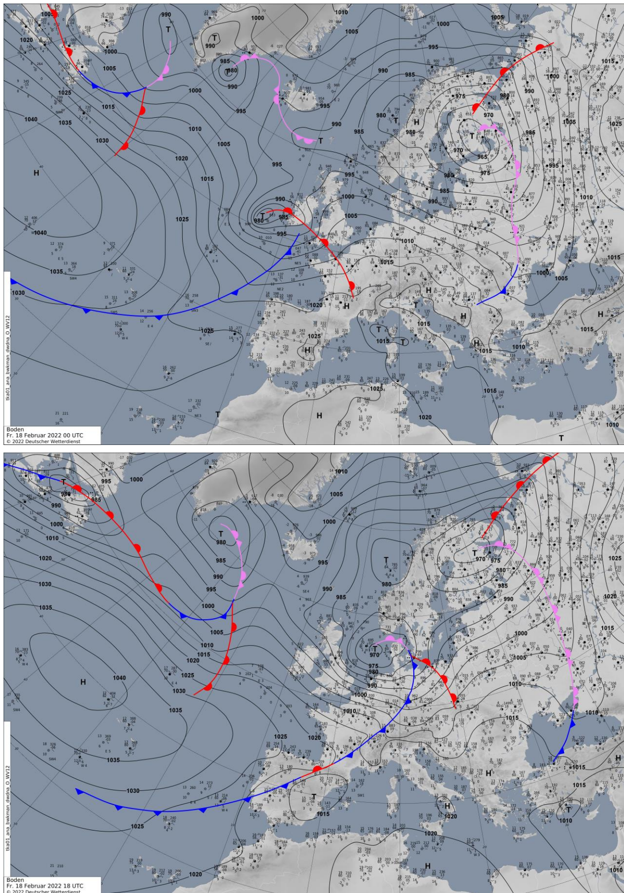
Figure 6: Surface pressure analysis, fronts and station recordings. Feb 18 2022, 06Z (top), Feb 18 2022, 18Z (bottom). Source: DWD
