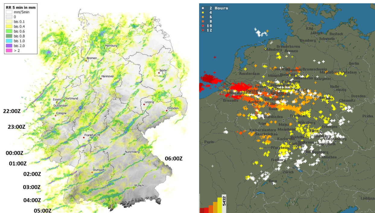
Figure 11: Propagation of the cold front of low pressure system “Antonia” on Feb 20-21 2022 in Germany based on hourly radar information (rain amount per 5 minutes, left). Lightning detection between Feb 20 2022, 18Z, and Feb 21 2022, 06Z. Data sources: DWD, www.blitzortung.org
