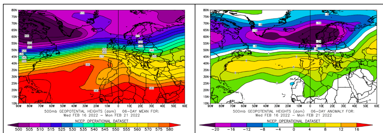
Figure 2: 500 hPa geopotential height (gpdam), left, and deviation from long term mean (1991-2020), right. 6 day-mean Feb 16-21 2022. Data: https://psl.noaa.gov
