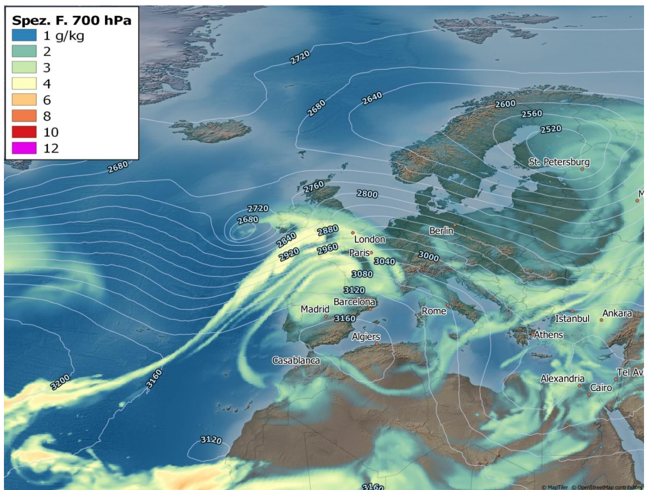
Figure 9: Analysis 700-hPa geopotential height (gpdam) and specific humidity (g/kg). Feb 18 2022, 00Z. Data: GEM
