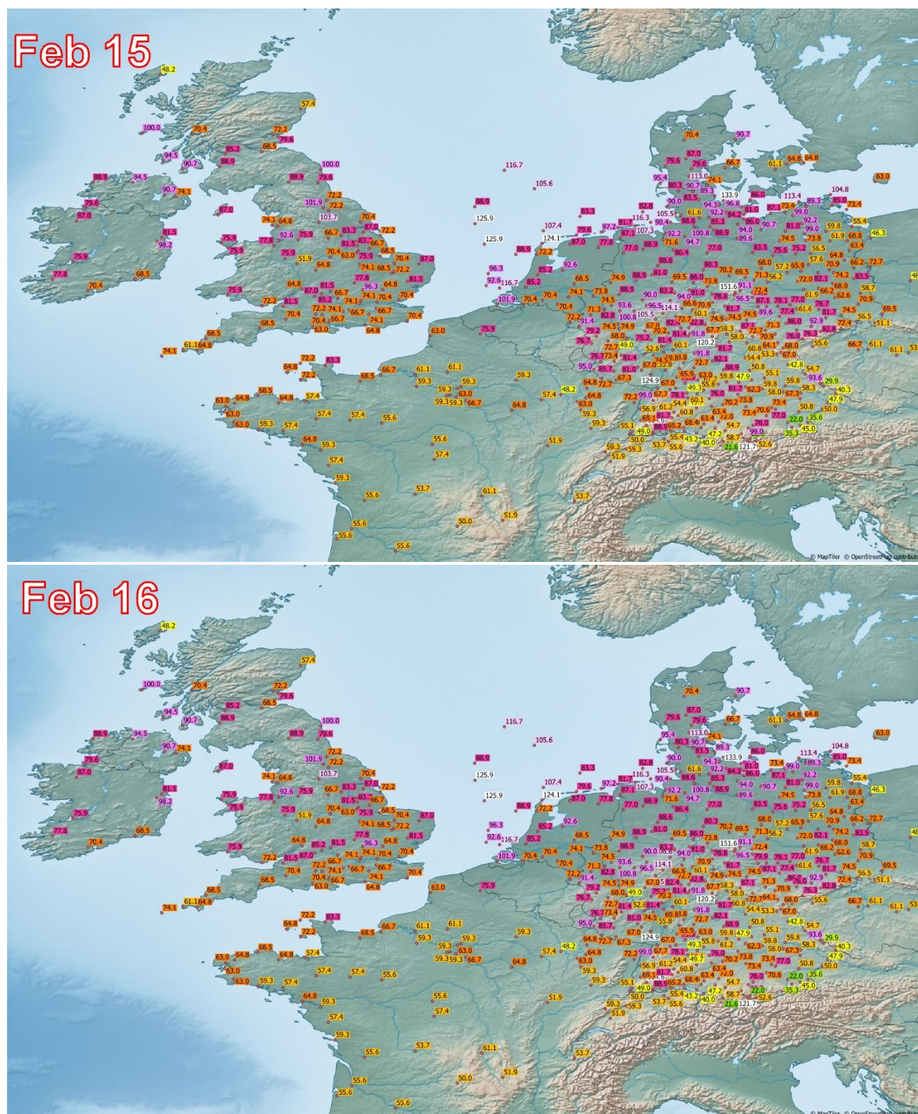
Figure 7a: Maximum wind gusts (German weather station network of DWD and METARS), Feb 15 2022 (top) and Feb 16 2022 (bottom). Data source: DWD and http://www.mesonet.agron.iastate.edu
