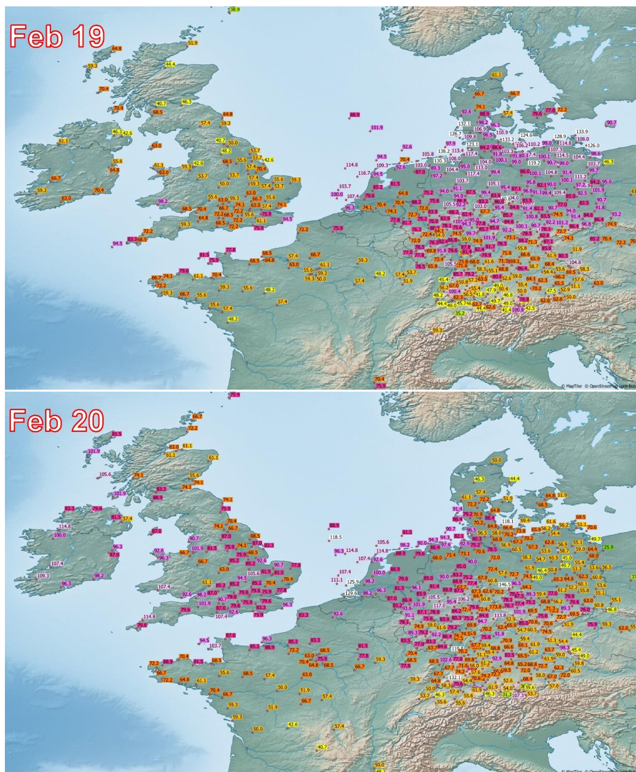
Figure 7c: Maximum wind gusts (German weather station network of DWD and METARS), Feb 19 2022 (top) and Feb 20 2022 (bottom). Data source: DWD and http://www.mesonet.agron.iastate.edu
