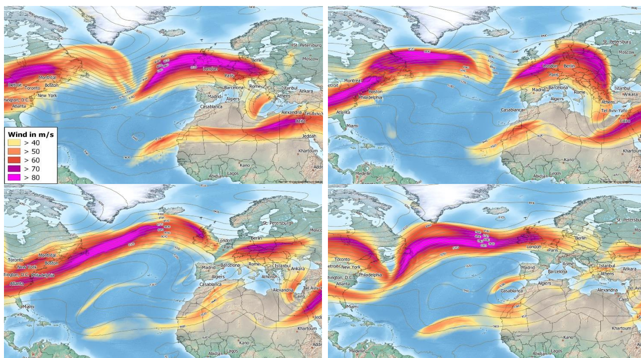
Figure 4: Analysis 300-hPa geopotential height (gpdam) and windspeed (m/s). Feb 17 2022, 12Z (upper left), Feb 18 2022, 12Z (upper right), Feb 19 2022, 12Z (bottom left), Feb 20 2022, 12Z (bottom right). Data: GEM
