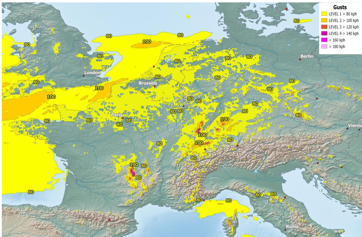
Maximum gusts in kph 13 March 2021. (INIT: 12 March 2021, 00 UTC. ICON-EU). Image: B. Mühr
